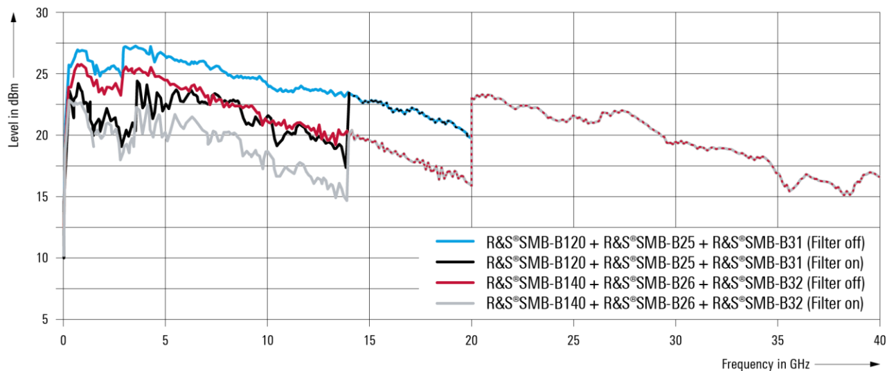
Maximum available output level versus frequency, Low Harmonic Filter off and on (meas.).
